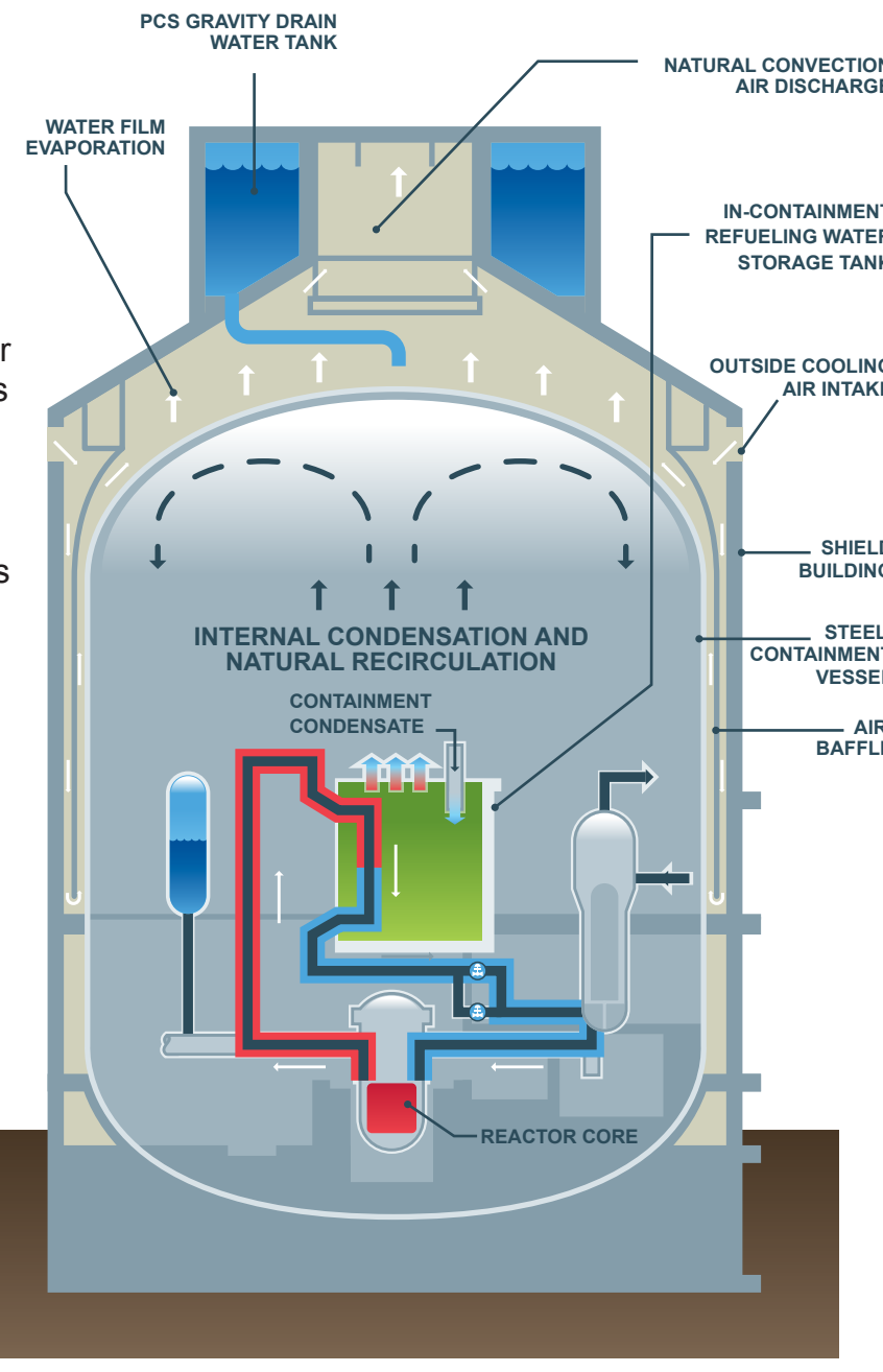
TRANSFER OF REACTOR DECAY HEAT TO OUTSIDE AIR
